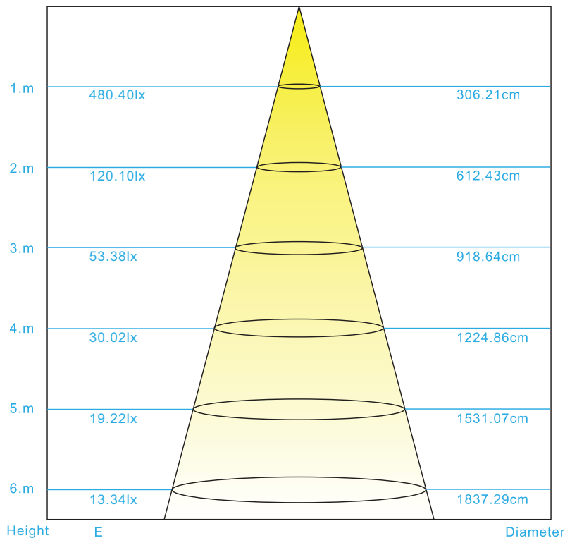
Beam Angle: 113.30°
