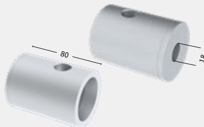
RECEIVER 203008
