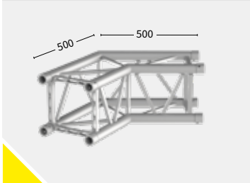
TPM29S-C204 120° 129504 6.6 kg
