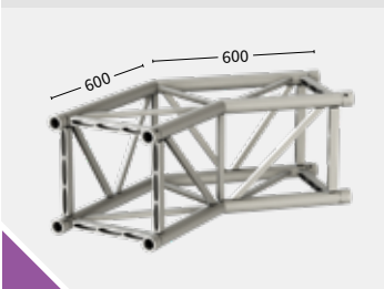
TPM39S-C205 135° 139505 9.6 kg
