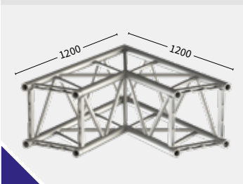
TPM39S-C202 60° 139502 14.6 kg
