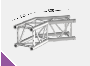
TPM29S-C205 135° 129505 7 kg
