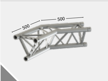
TPM29T-C205 135° 126505 4.63 kg
