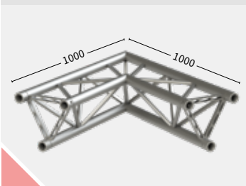
TPM29T-C202 60° 126502 7.11 kg
